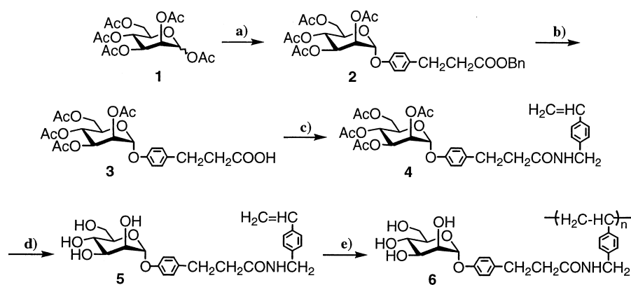
a) TMSOTf, HO-C 6 H 4 -CH 2 CH 2 COOBn ( 34 ) / CH 2 Cl 2 , 0 °C (y. 83%); b) 10% Pd(OH) 2 -C, H 2 / EtOH, rt (y. 97%); c) H 2 N-CH 2 -C 6 H 4 -CH 2 =CH 2 , WSC / CH 2 Cl 2 , 0 °C (y. 73%); d) NaOMe / MeOH, rt (y. 97%); e) AIBN / DMSO, 65 °C, 24 h (y. 98%).
